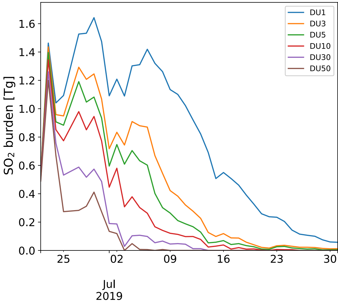
(a) TROPOMI
