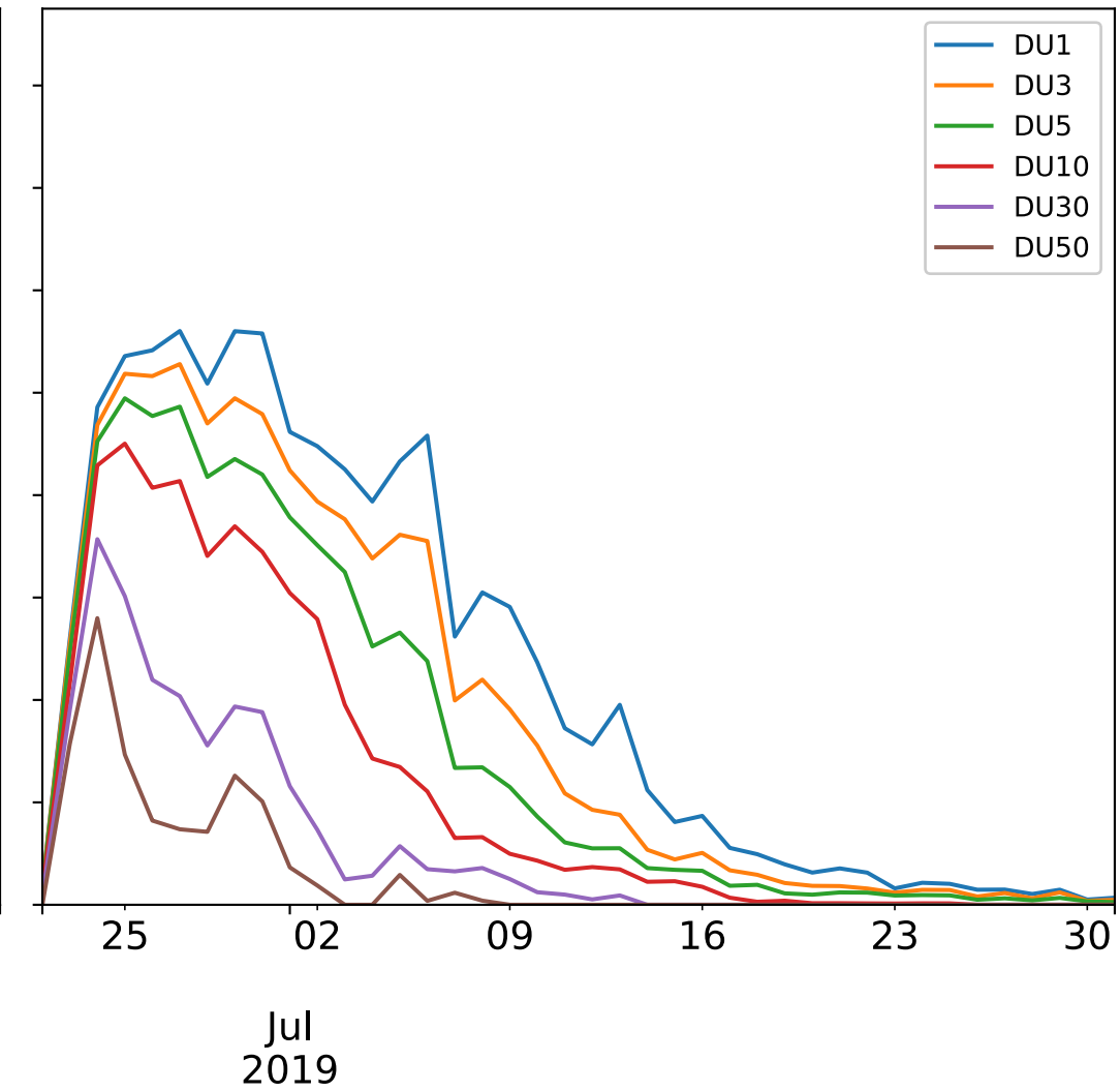
(b) GOME-2B
