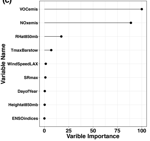
(c) Variable Importance of Ozone SVR model
