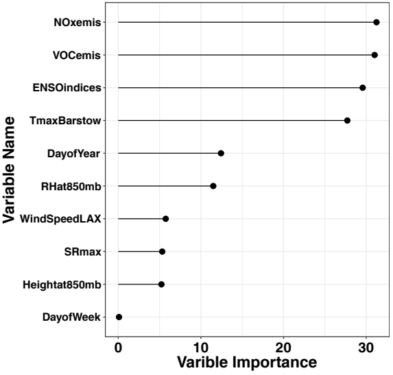
Variable Importance of Ozone RF model
