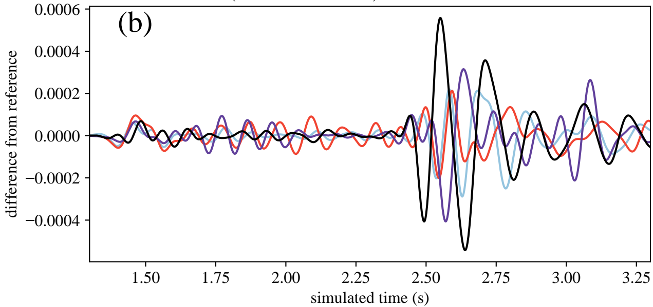
Difference (MLxtri-reference) at receiver with 2 km offset
