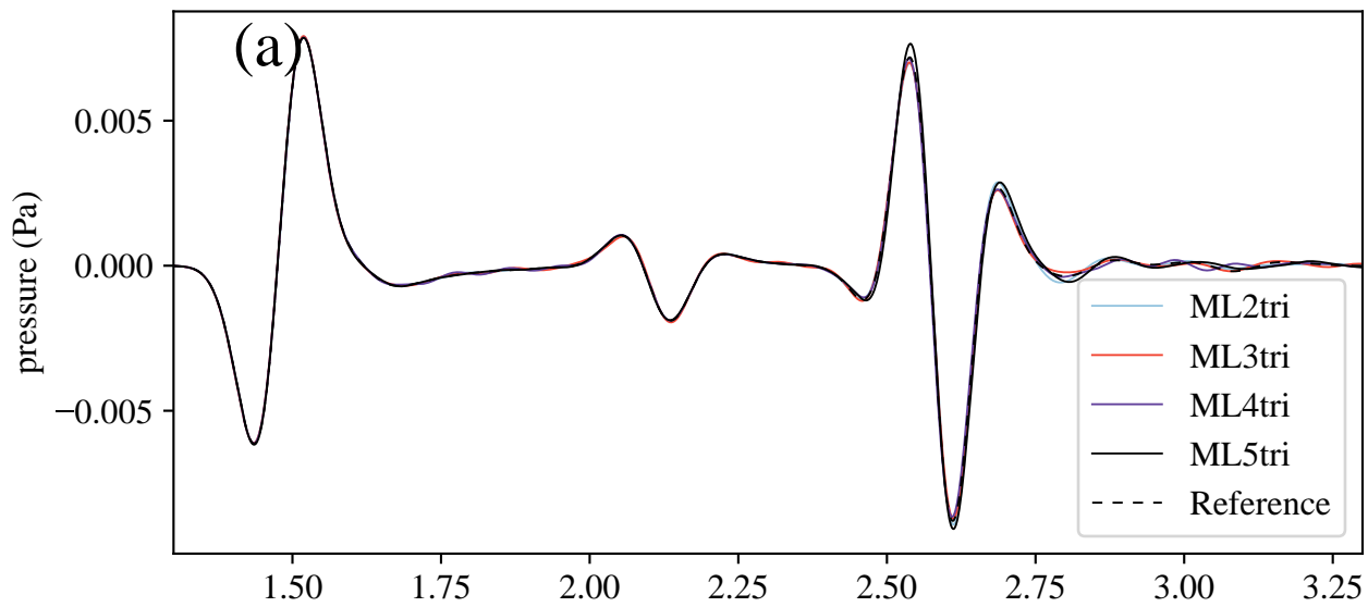
Pressure at receiver with 2 km offset
