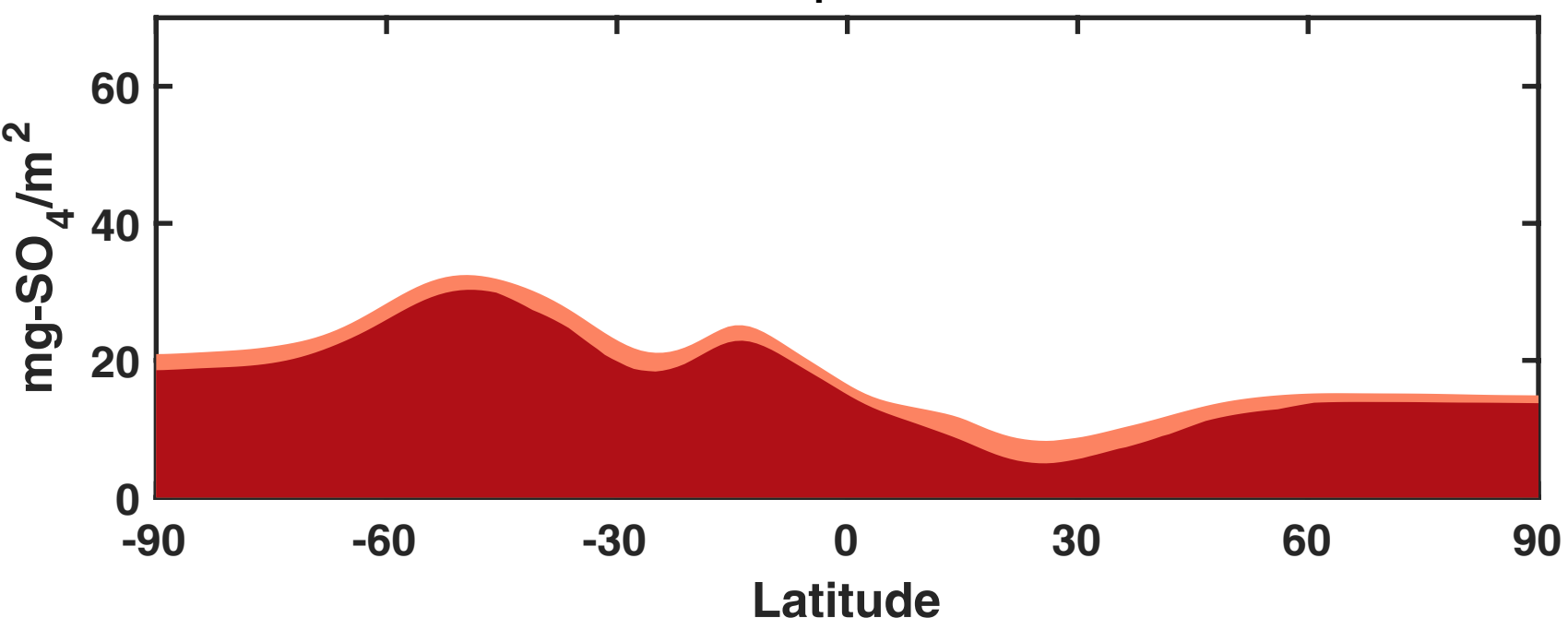
(b) Total column SO 4 increase [2035-2054]
