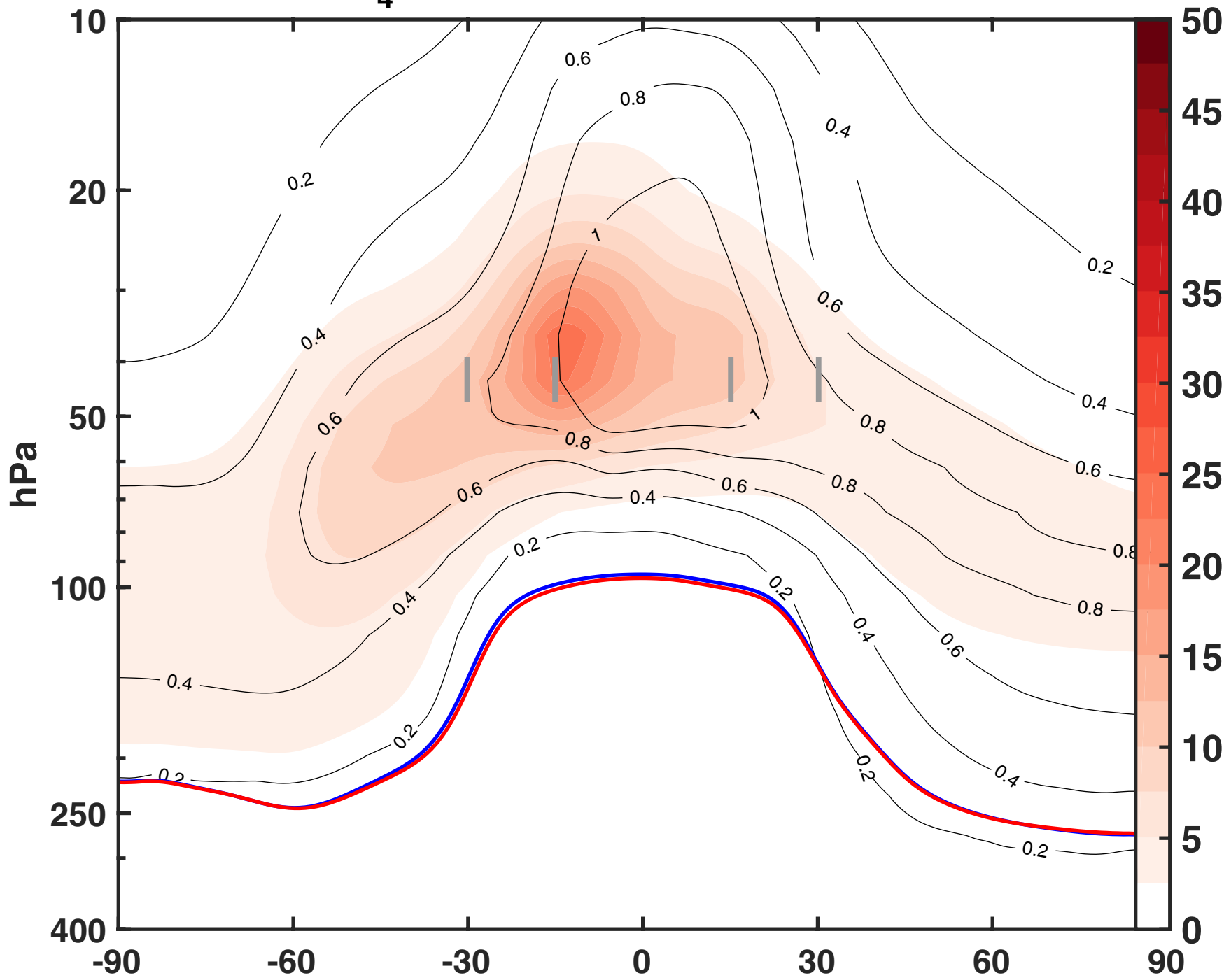
(a) SO 4 increase (μg-S/kg air) [2035-2054]
