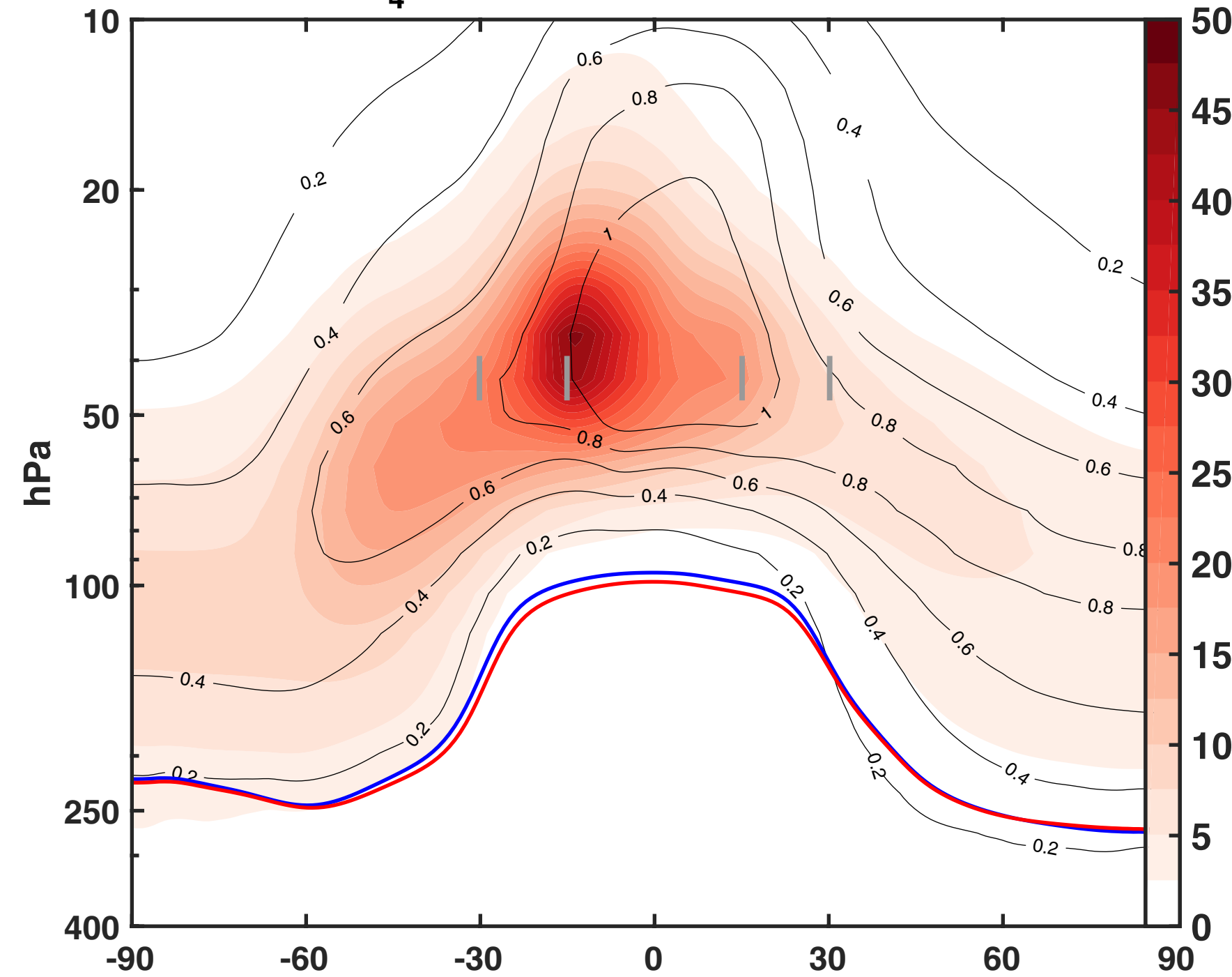
(c) SO 4 increase (μg-S/kg air) [2050-2069]
