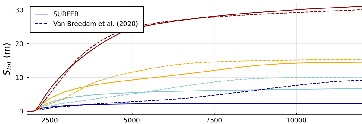
(a) Total sea level rise
