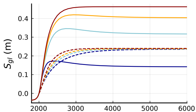
(c) Glacier contribution to sea level rise
