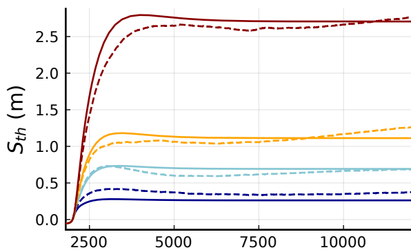
(b) Ocean thermal expansion
