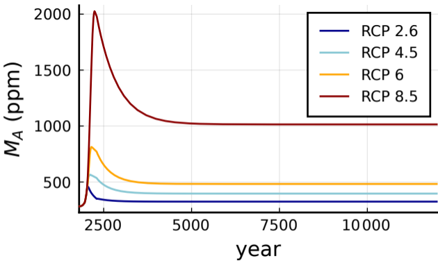
(a) Atmospheric CO 2 concentration
