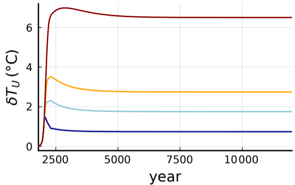
(b) Global mean temperature anomaly
