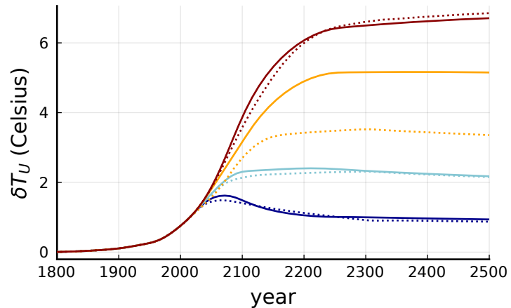
(b) Global mean temperature anomaly
