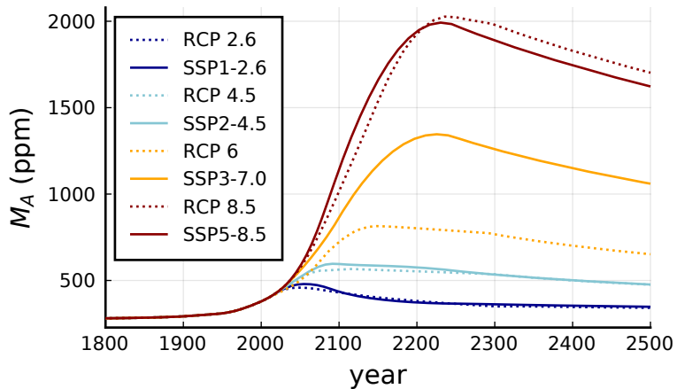
(a) Atmospheric CO 2 concentration
