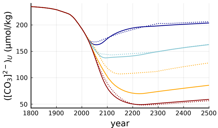
(f) Upper ocean layer carbonate concentration
