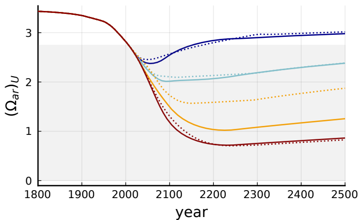
(e) Upper ocean layer aragonite saturation state
