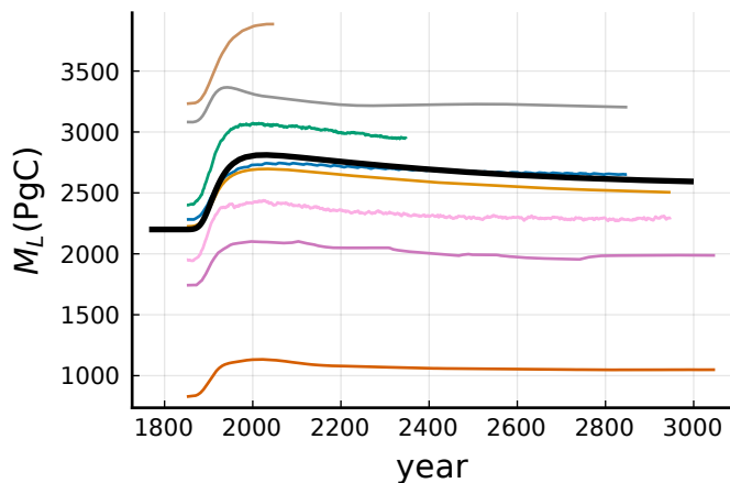
(e) Carbon in land reservoir
