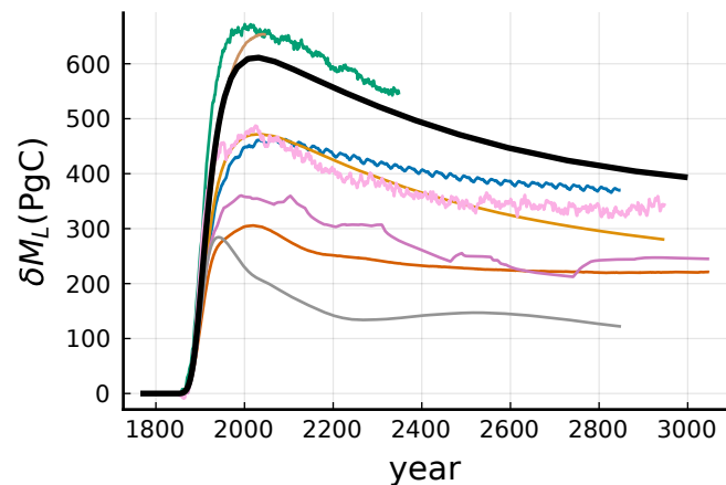
(f) Carbon anomaly in land reservoir
