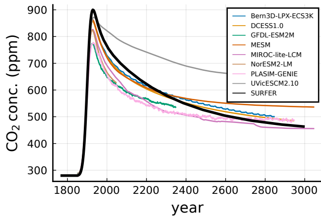
(a) Atmospheric CO 2 concentration
