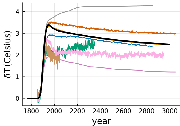
(b) Global mean temperature anomaly
