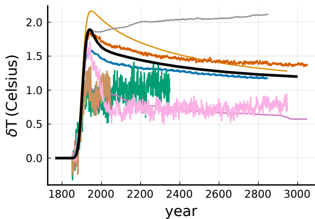
(b) Global mean temperature anomaly
