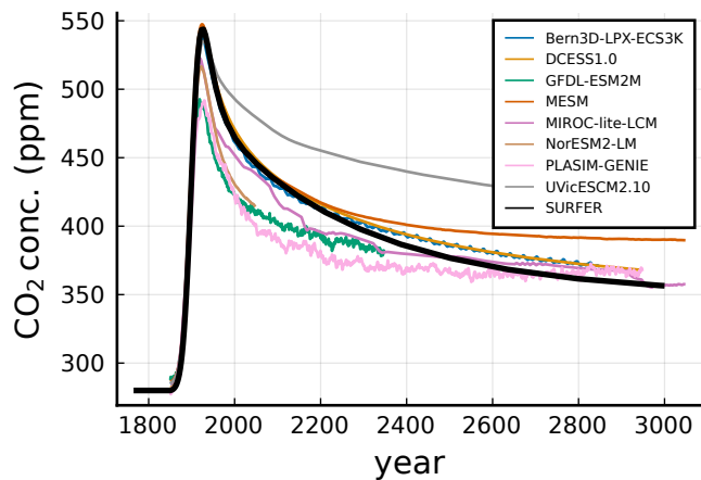
(a) Atmospheric CO 2 concentration
