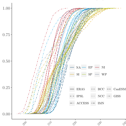
Tropopause temperature (K)
