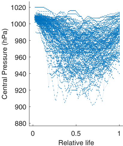
Historical (IBTrACS)
