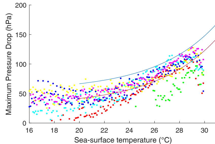
(b) Sea-surface temperature and maximum pressure drop
