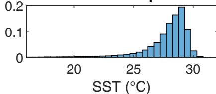
Sea-surface temperature
