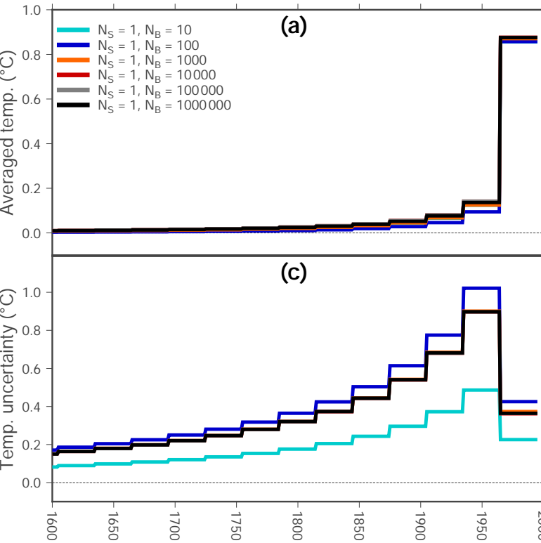
Artificial Profile
