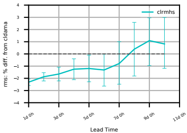
(a) T01to30
