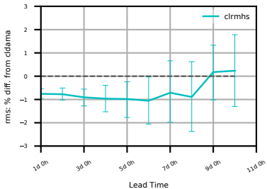
(c) U
