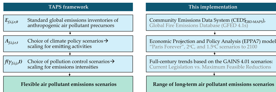
Figure 1. Summary of the Tool for Air Pollution Scenarios (TAPS) framework and implementation here, based on climate policy scenarios in EPPA7 and pollution control scenarios from the Greenhouse Gas–Air Pollution Interactions and Synergies (GAINS) model. Emissions trends are specific to each fuel f , pollutant species i , sector j , region r , and time point t in the inventories and EPPA7 scenarios used.
