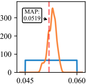
Dalton Number PDF
