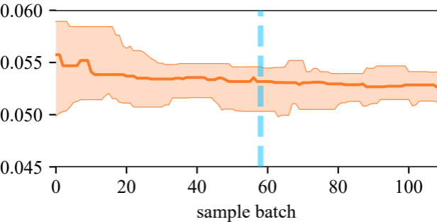
Dalton Number
