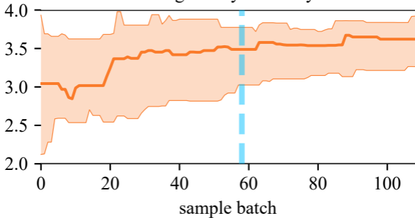
Smagorinsky Viscosity
