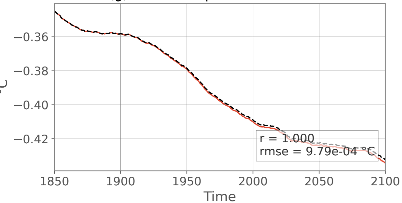
(g) Global temperature at 4000 m
