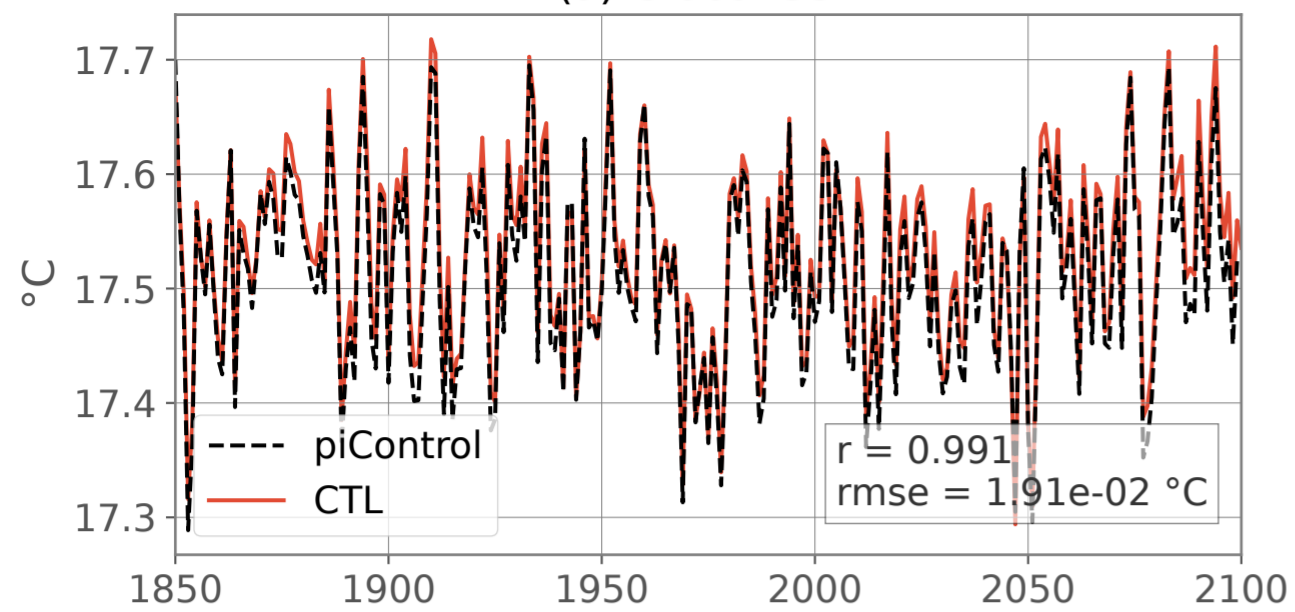
(c) Global temperature at 500 m
