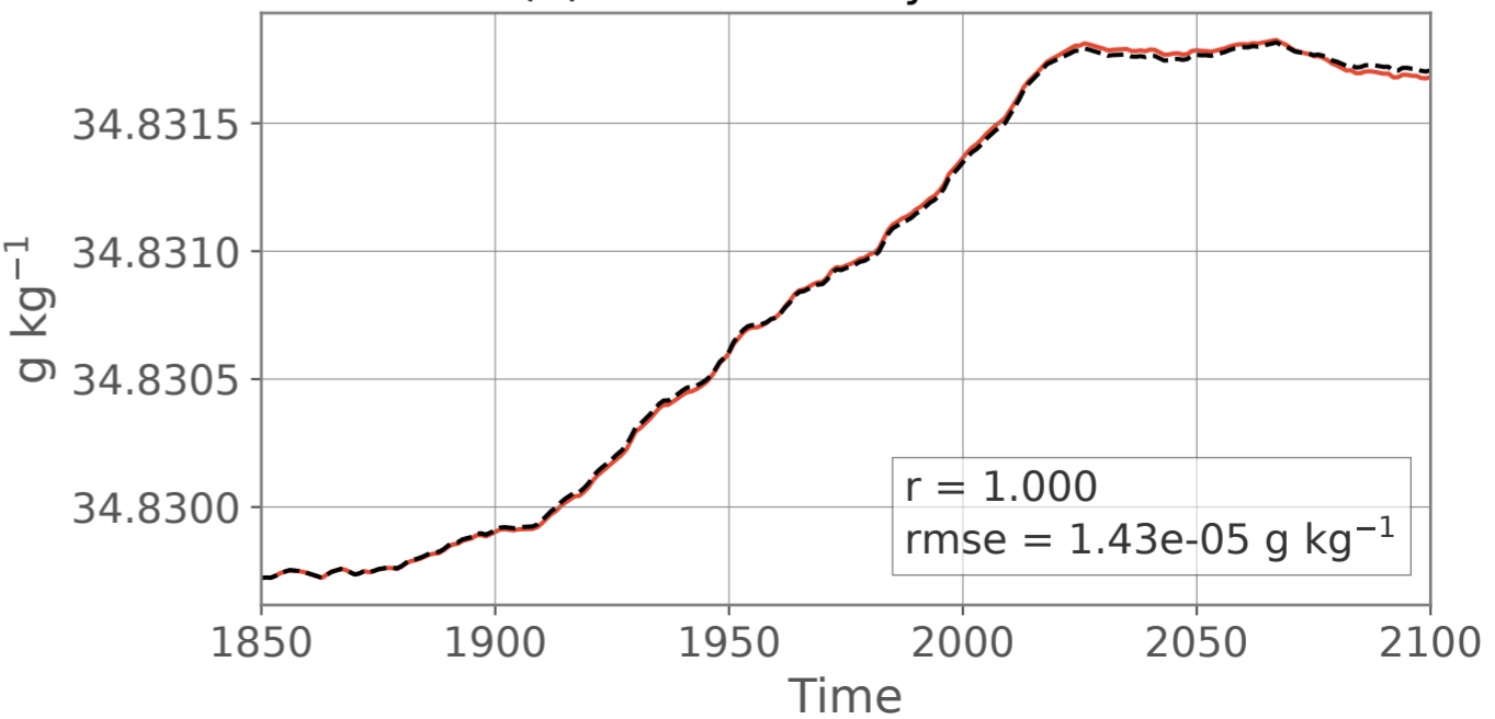
(h) Global salinity at 4000 m
