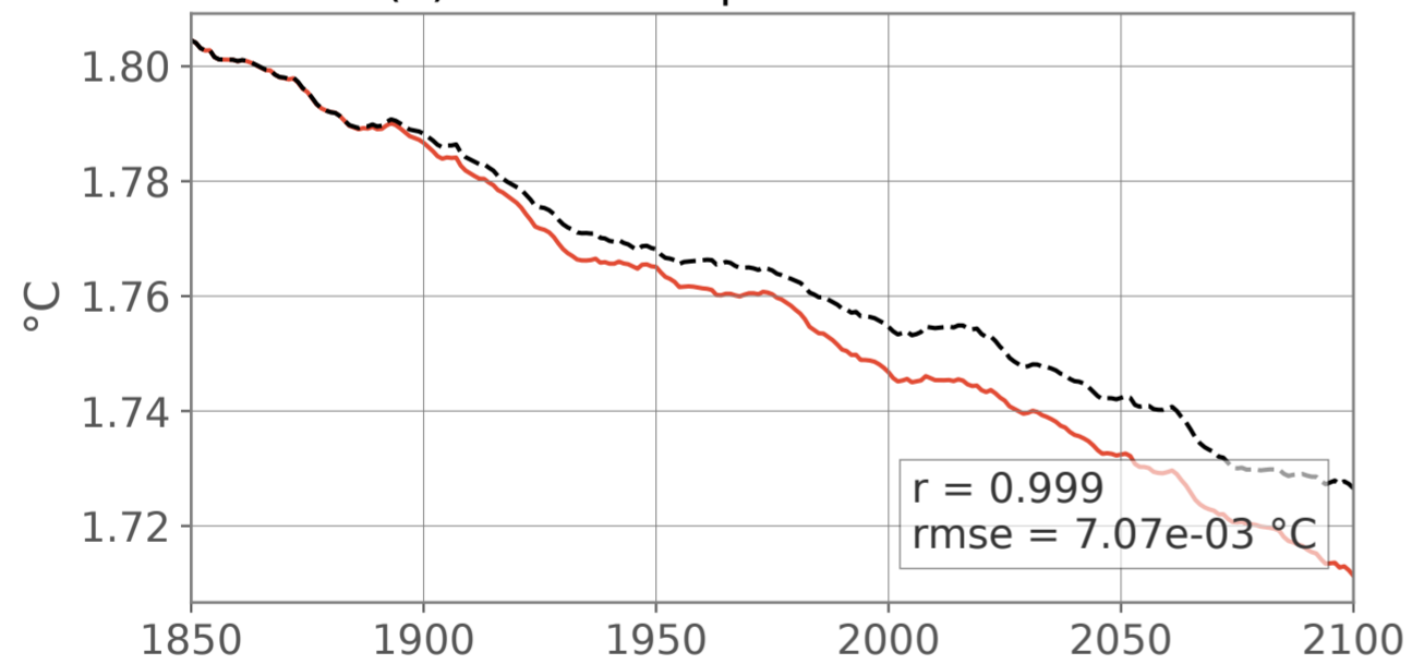
(g) Global temperature at 4000 m
