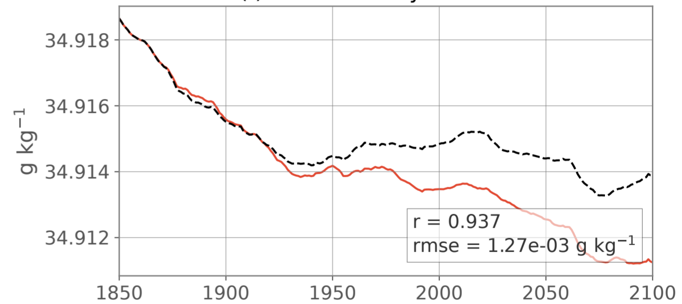
(h) Global salinity at 4000 m
