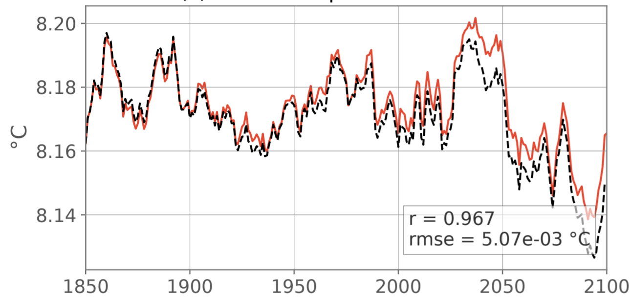
(e) Global temperature at 2000 m
