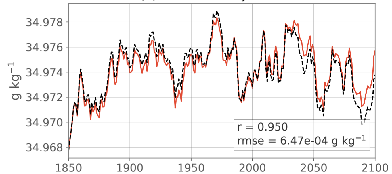
(f) Global salinity at 2000 m
