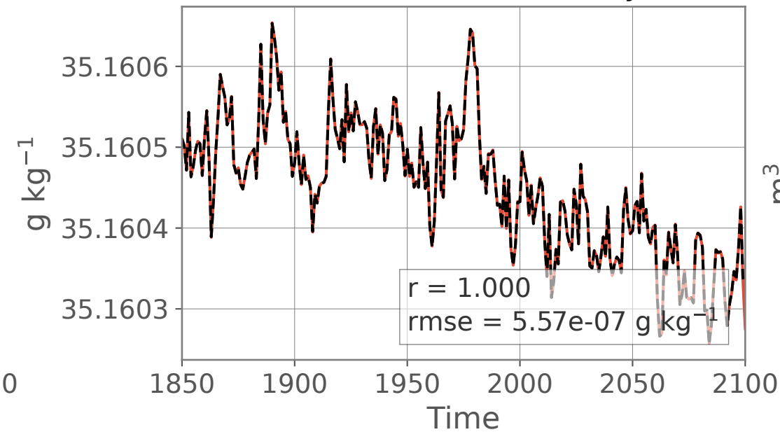
(e) Global mean salinity
