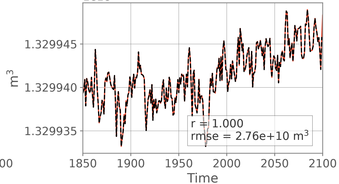
(f) Global ocean volume
