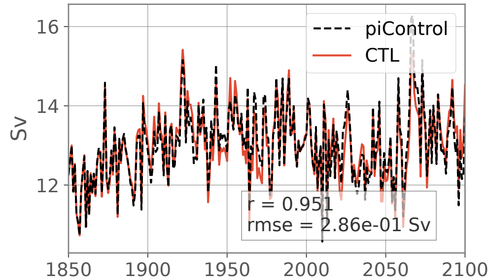
(a) Max AMOC 10-60°N, >500 m
