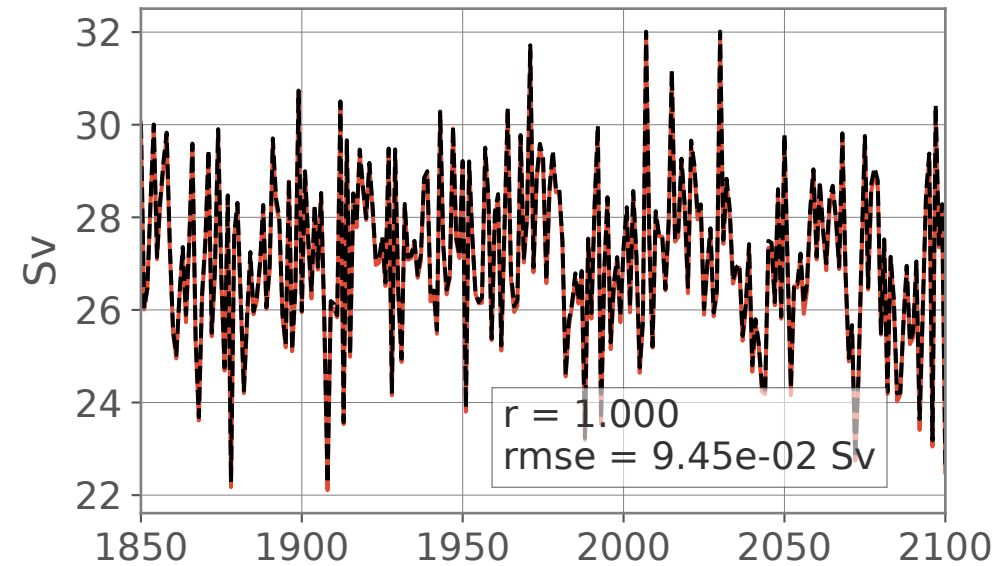
(b) Max Deacon cell 80-30°S, <2000 m
