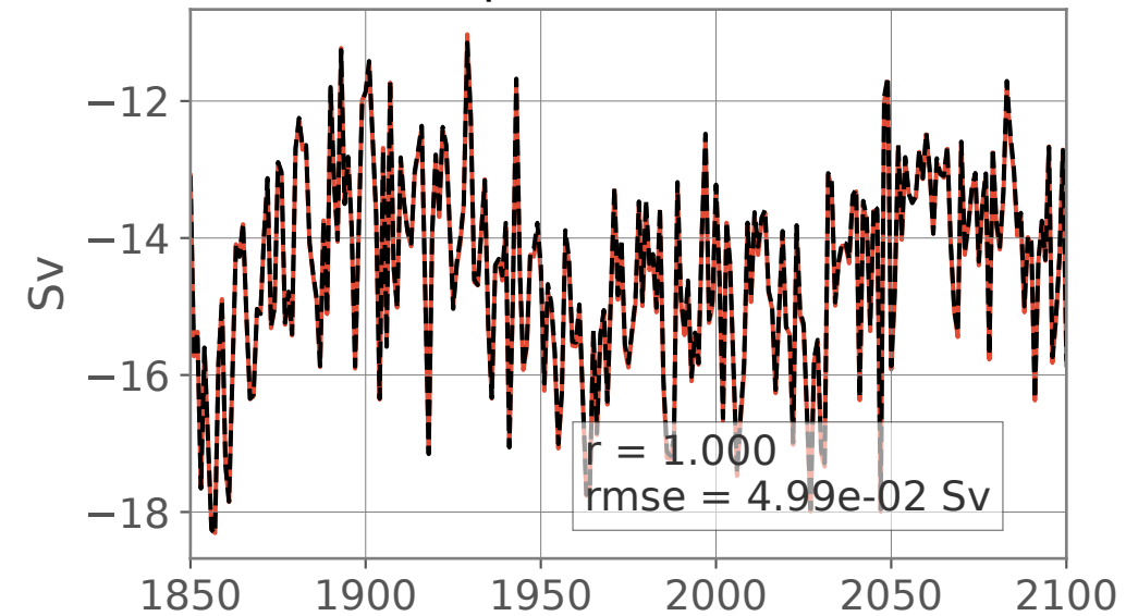
(c) Max deep cell 80-30°S, >2000 m
