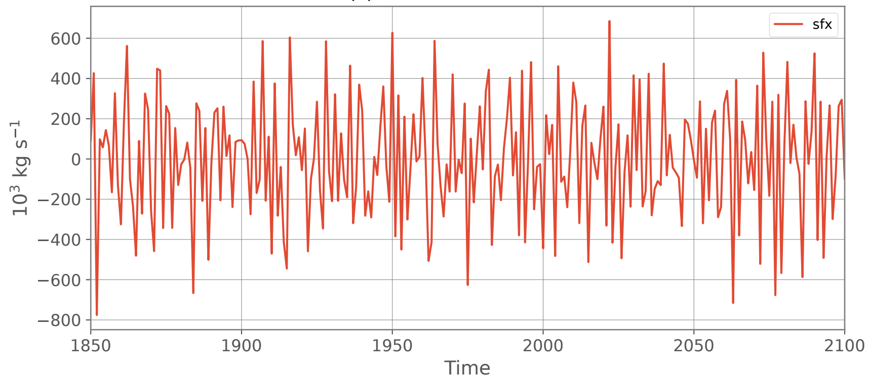
(c) Global mean salt flux
