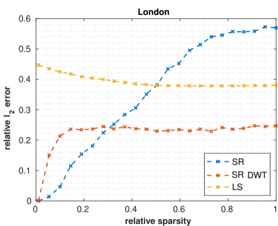
(a) \frac{m}{n} \approx 50\%
