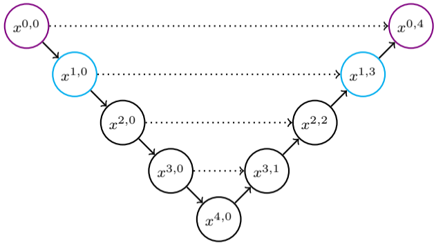
(a) U-Net
