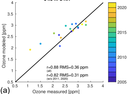
54.0 hPa NH
