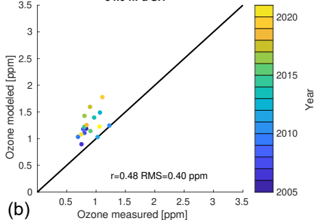
54.0 hPa SH
