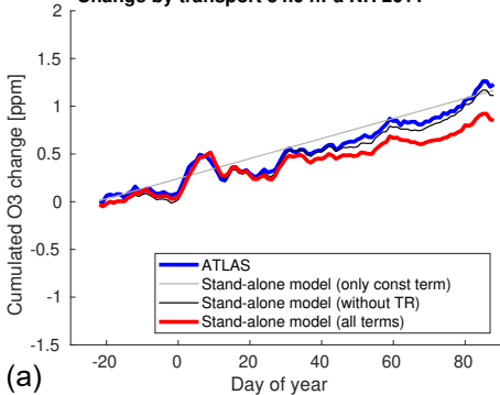
Change by transport 54.0 hPa NH 2011
