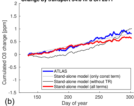
Change by transport 54.0 hPa SH 2011
