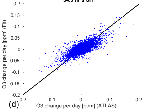
54.0 hPa SH
