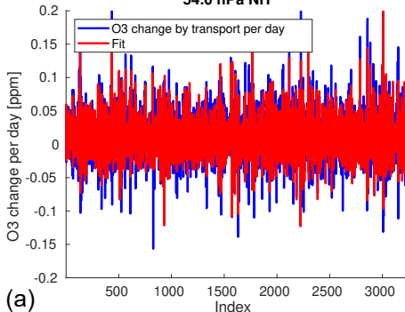
54.0 hPa NH
