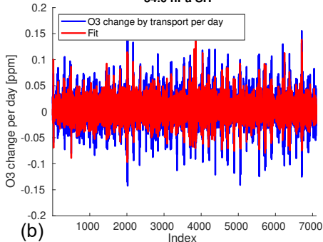
54.0 hPa SH
