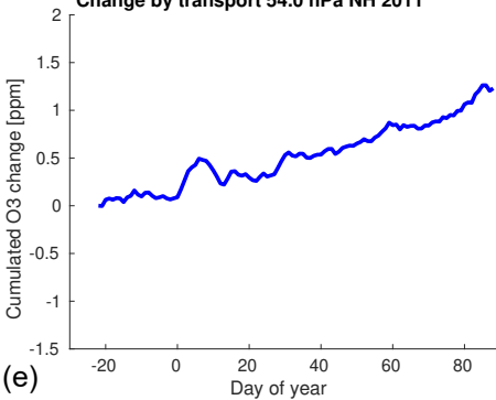
Change by transport 54.0 hPa NH 2011
