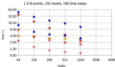
(c) Juwels-Booster: Time to solution for components
