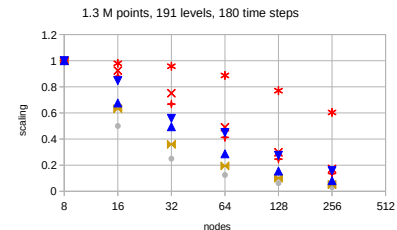
(f) Levante: Cumulative strong scaling of components
