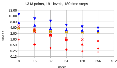
(e) Levante: Time to solution for components
