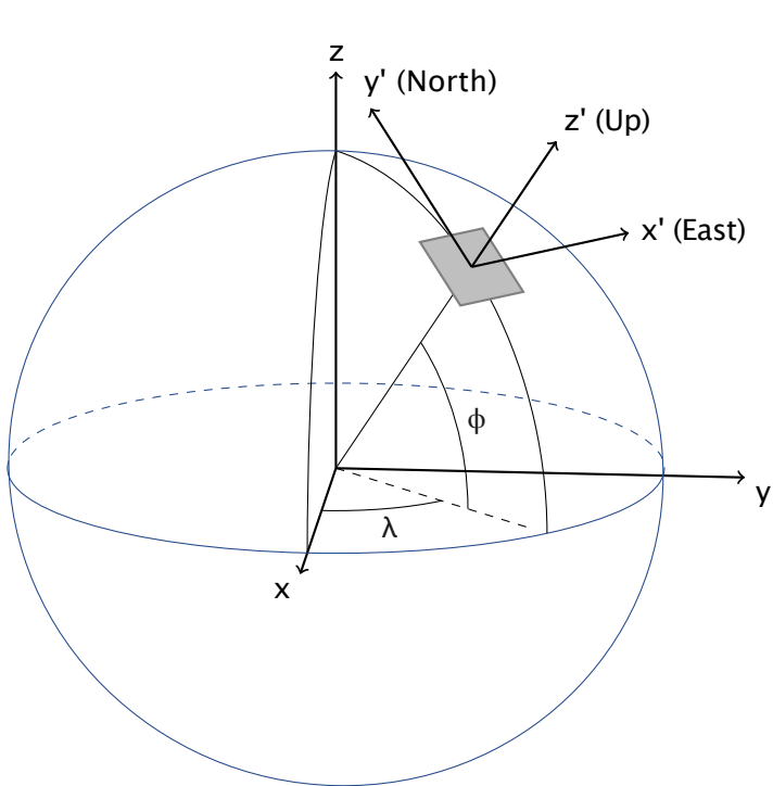
(a) Geodetic, ECEF and global ENU coordinates
