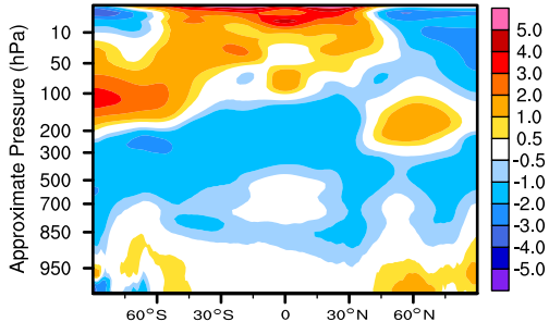
(b) CLIM — ERA5 (unit: K)
