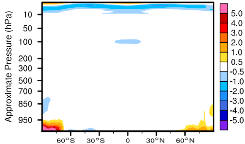
(a) ERAI — ERA5 (unit: K)
