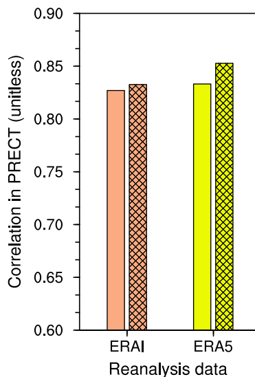
(e) Nudged to ERAI or ERA5
