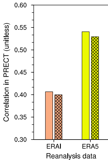
(b) Nudged to ERAI or ERA5
