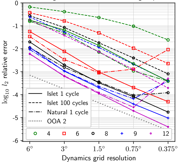
Islet method stability: divergent flow, Gaussian hills, long steps
