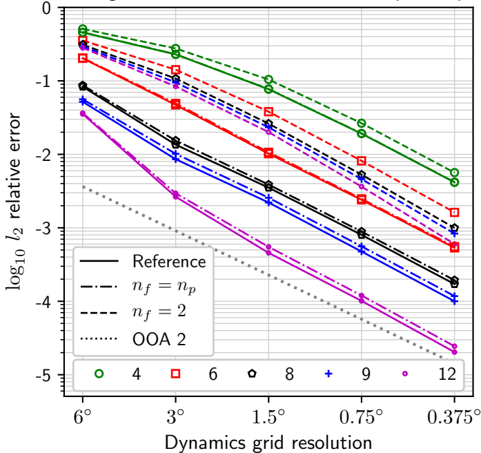
Physics grid source term accuracy: nondivergent flow, Gaussian hills, short steps, midpoint
