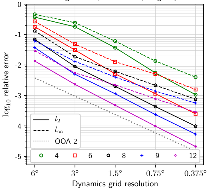
Islet method accuracy: divergent flow, cosine bells, long steps
