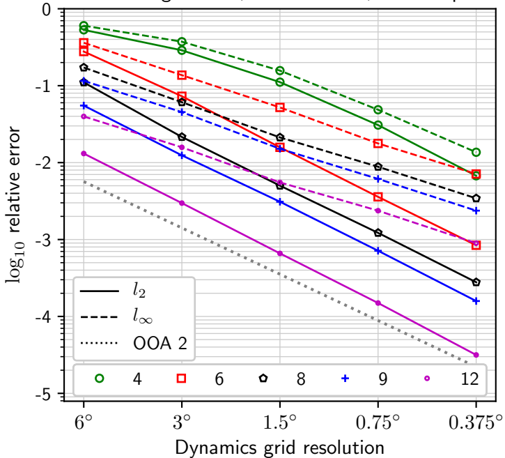
Islet method accuracy: nondivergent flow, Gaussian hills, short steps
