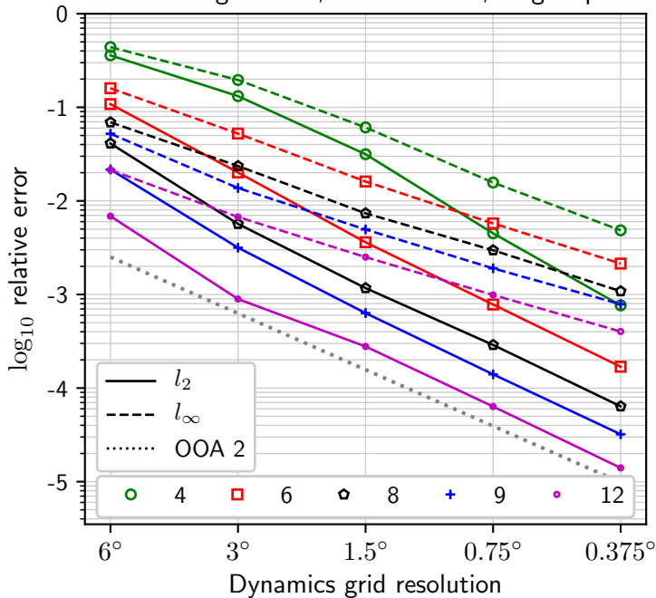
Islet method accuracy: nondivergent flow, Gaussian hills, long steps
