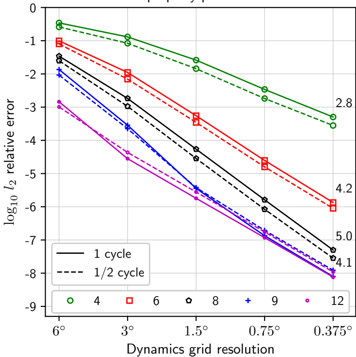
Trajectory interpolation: nondivergent flow, Gaussian hills, long steps, no property preservation
