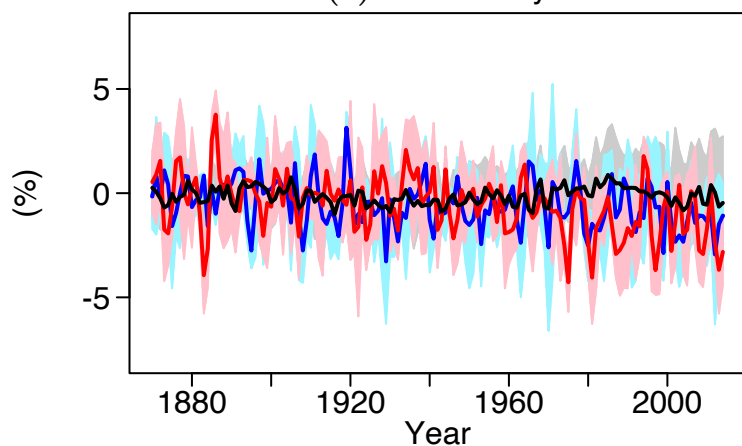
(e) PP anomaly
