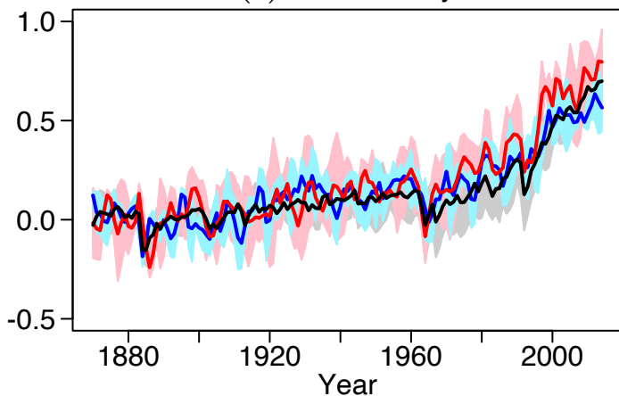
(c) O 2 (100 – 600 m) anomaly
