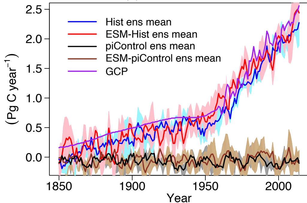
(b) air – sea CO 2 flux
