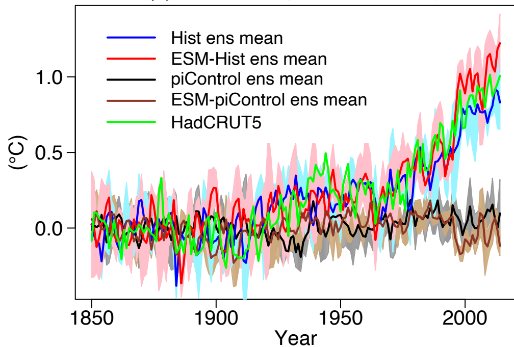
(c) Surface temperature anomaly
