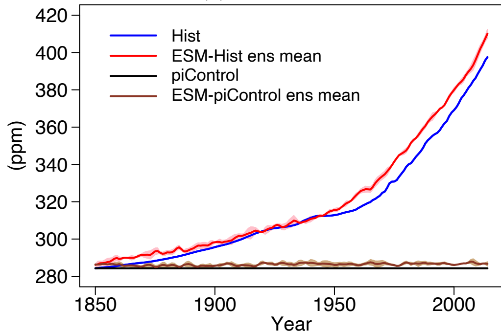
(a) Atmospheric CO 2
