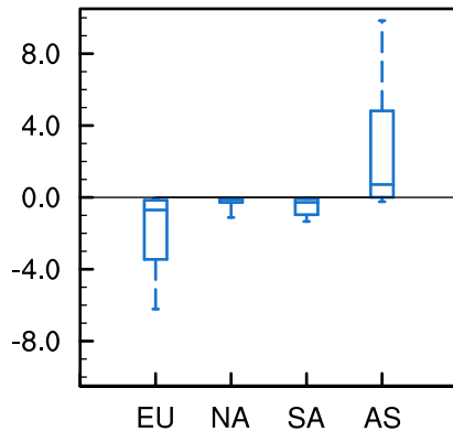
(e) OH^{tra}
