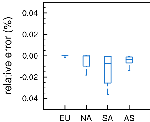
(a) O_3
