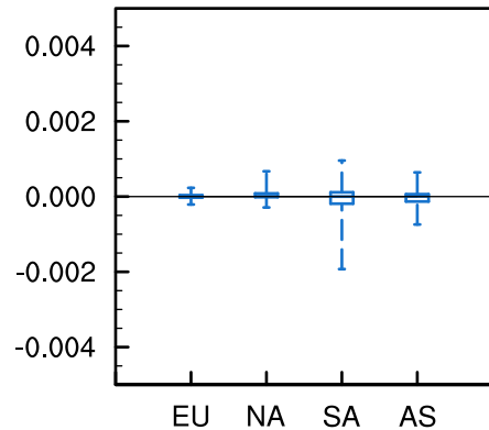
(c) flxn( O_3 )
