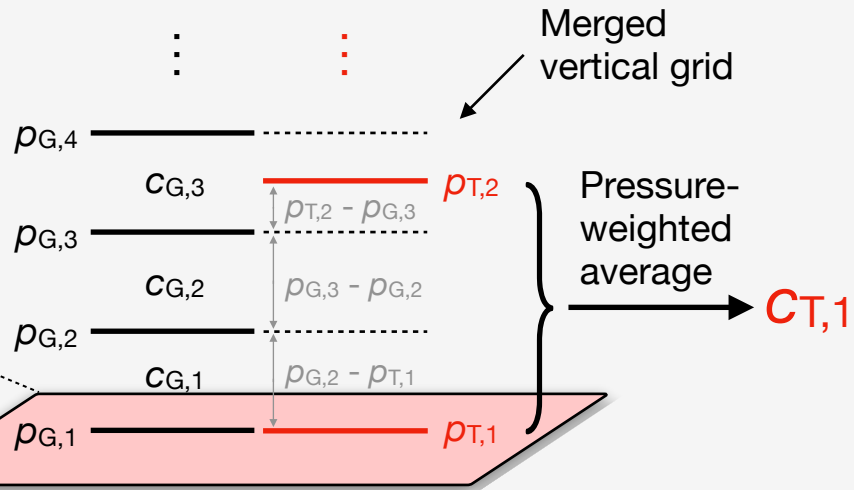
(b) Remap GEOS-Chem CH 4 profile to TROPOMI pressure grid
