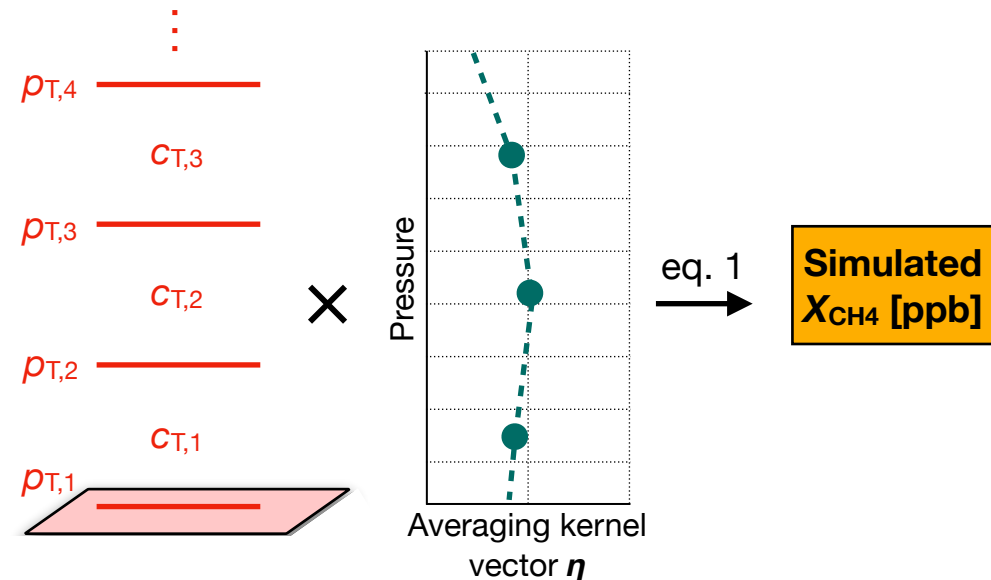
(c) Infer TROPOMI X CH 4 in GEOS-Chem atmosphere
