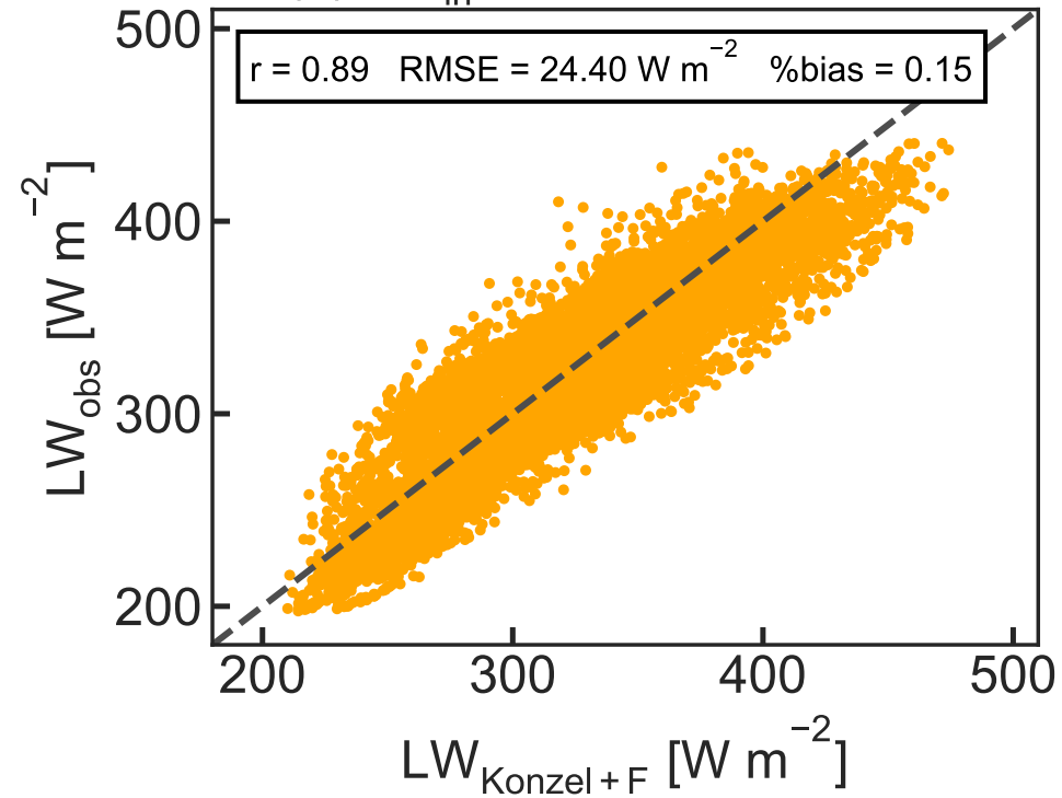
(a) LW_{in} after Konzelmann+F
