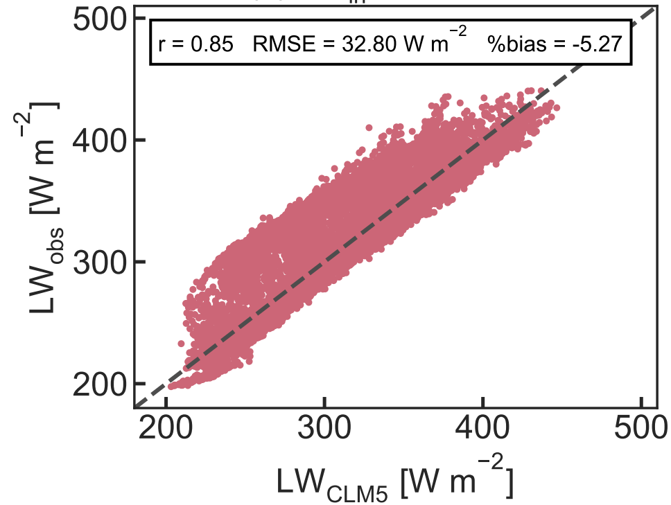
(b) LW_{in} after CLM5
