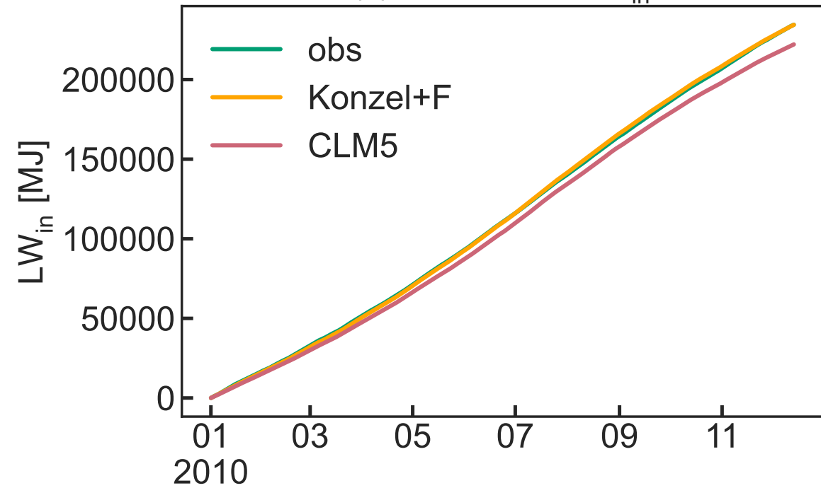
(c) Cumulative LW_{in}
