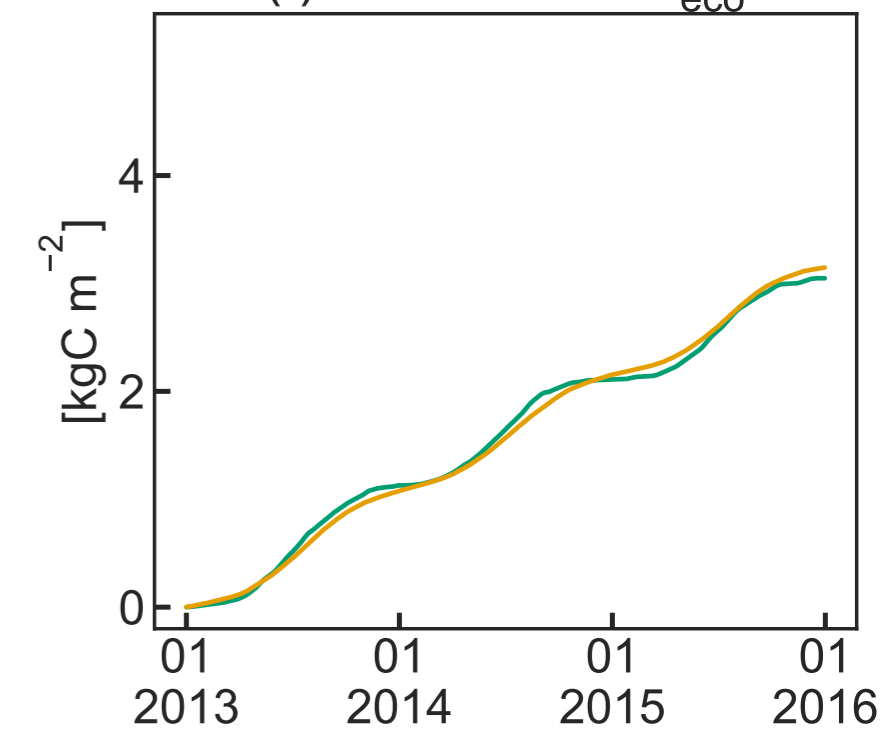
(f) Cumulative R_{eco}
