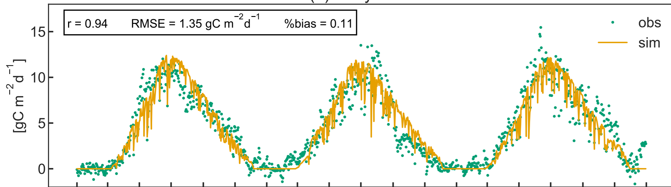
(c) Daily NEE
