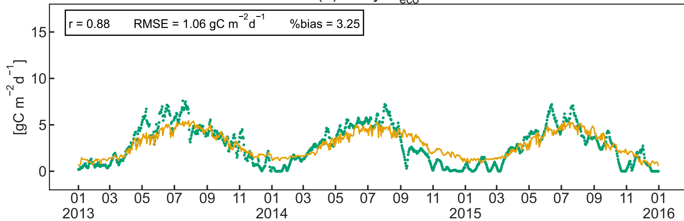
(e) Daily R_{eco}
