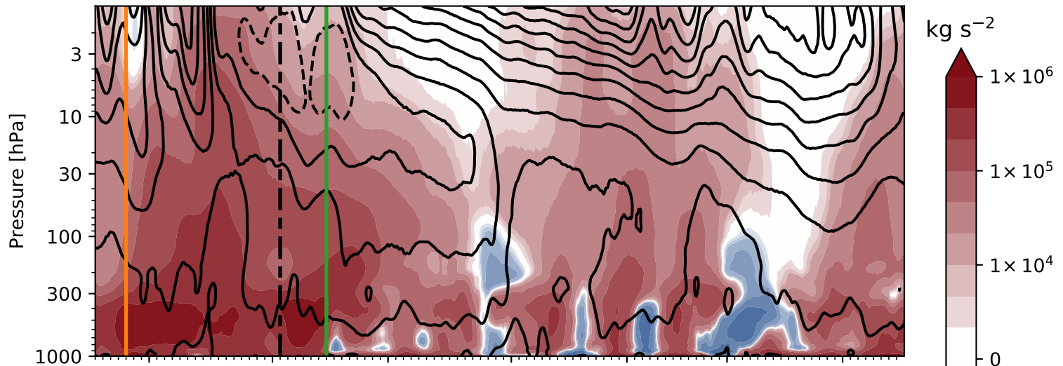
(b) 2018-19 U 60° N, F_z 50°-70° N: wave number 2
