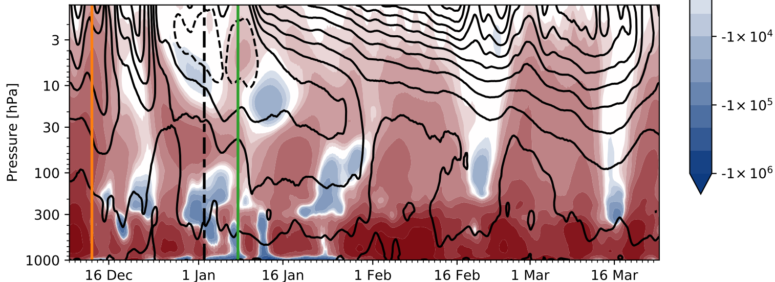
(b) 2018-19 U 60° N, F_z 50°-70° N: wave number 2
