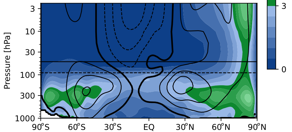
(c) control: U [m/s]
