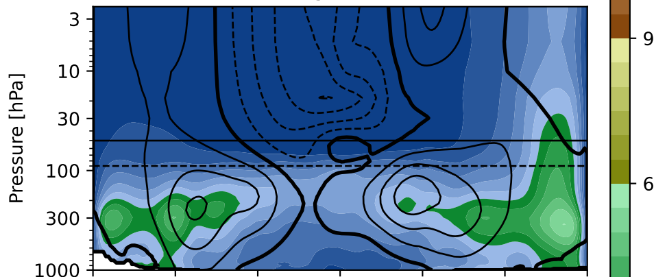
(c) control: U [m/s]
