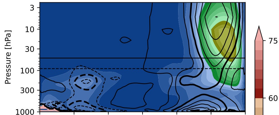
(e) nudged: V'T' [K m/s]
