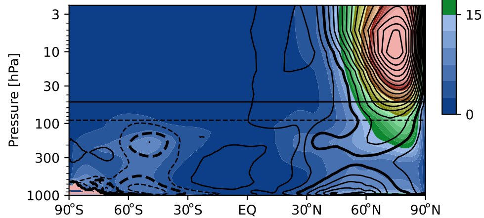
(f) control: V'T' [K m/s]
