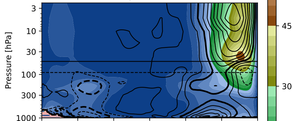
(f) control: V'T' [K m/s]
