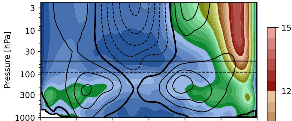
(b) nudged: U [m/s]
