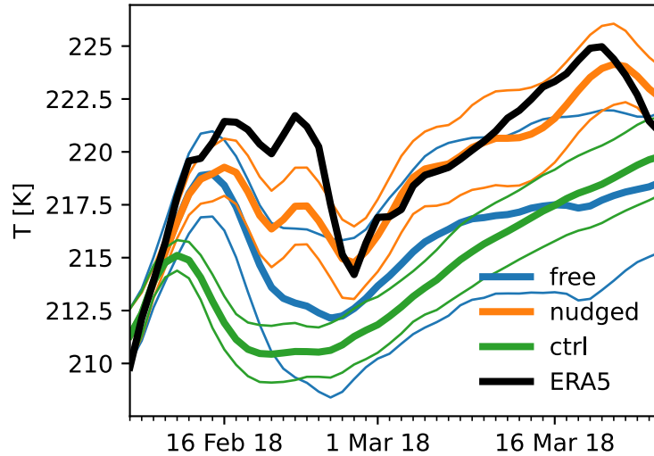
(b) T 155 hPa, 70° -90° N
