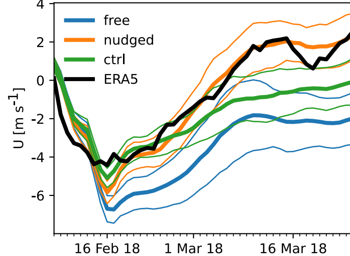
(c) U 80 hPa, 5° S - 5° N
