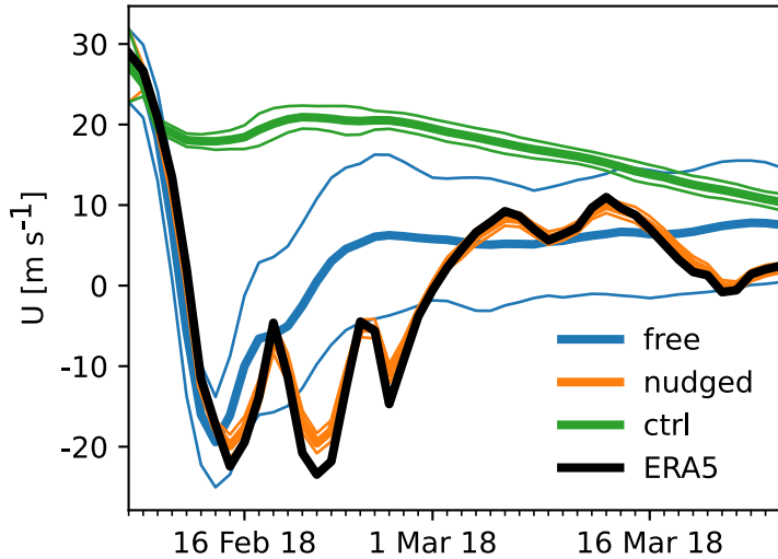
(a) U 10 hPa, 60° N
