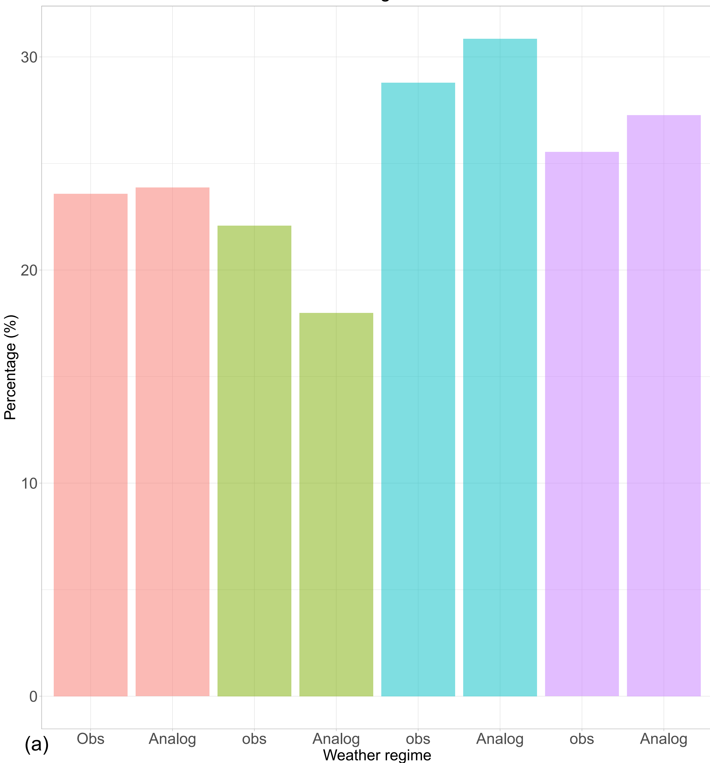
Weather regimes JJA
