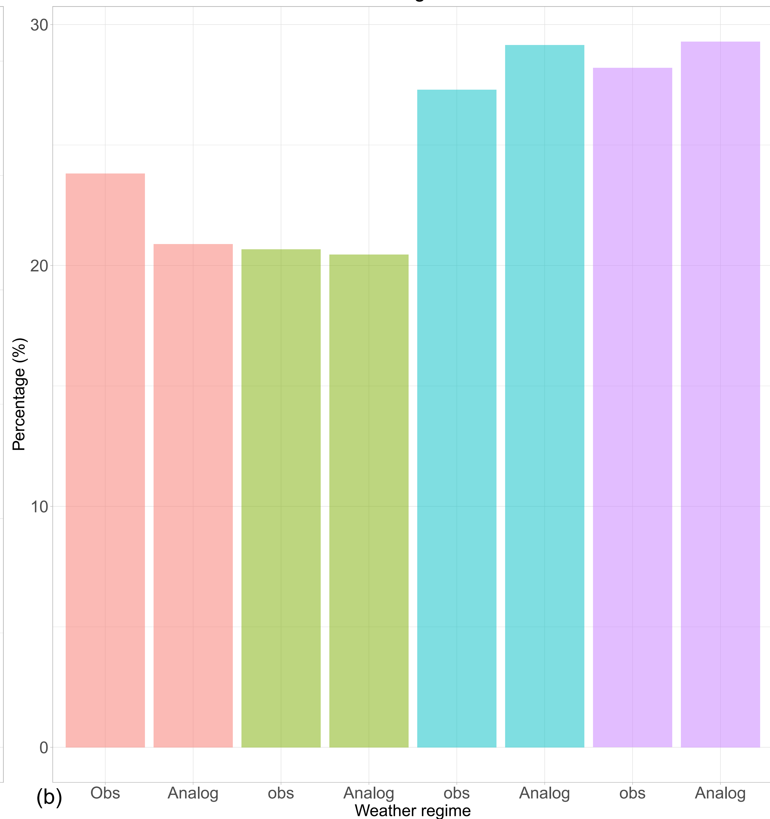
Weather regimes DJF
