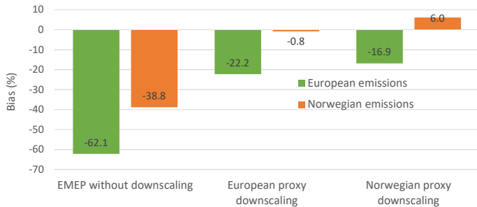
PM 2.5 bias for European and Norwegian, emissions and proxies
