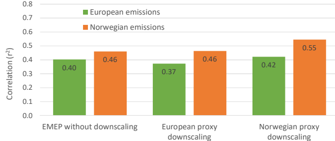
PM 10 r 2 for European and Norwegian, emissions and proxies
