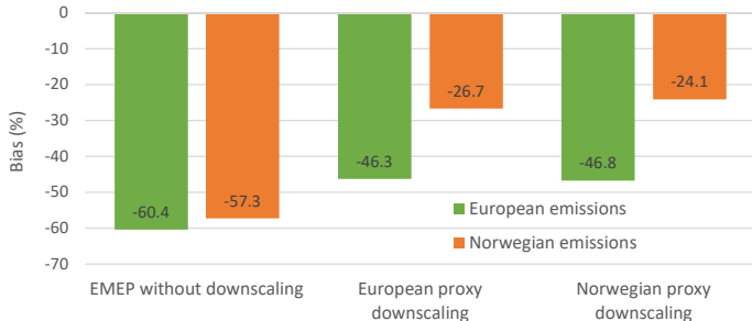
PM 10 bias for European and Norwegian, emissions and proxies
