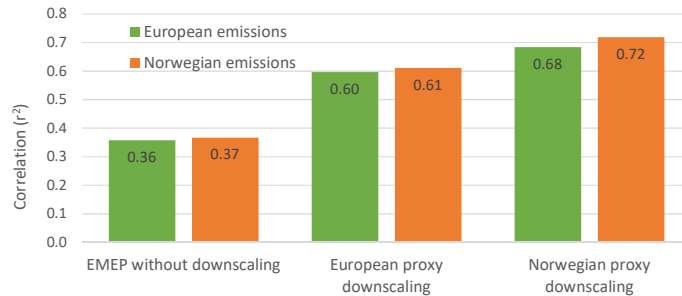
PM 2.5 r 2 for European and Norwegian, emissions and proxies
