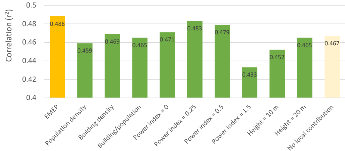
PM 2.5 r 2 for residential combustion proxy parameters
