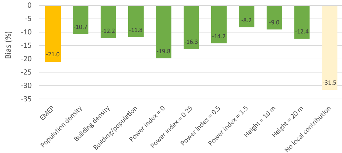
PM 2.5 bias for residential combustion proxy parameters
