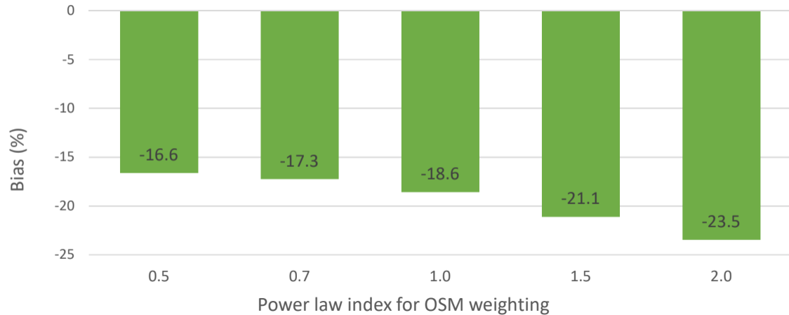
NO 2 bias due to changes in OSM power law weighting
