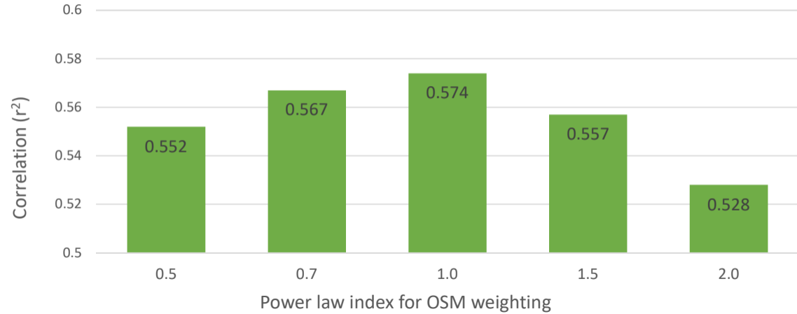
NO 2 r 2 due to changes in OSM power law weighting
